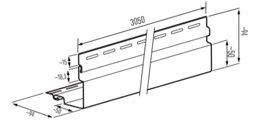
SV (P) 12V Outside corner for vertical installation (only for SV(P) 05)
