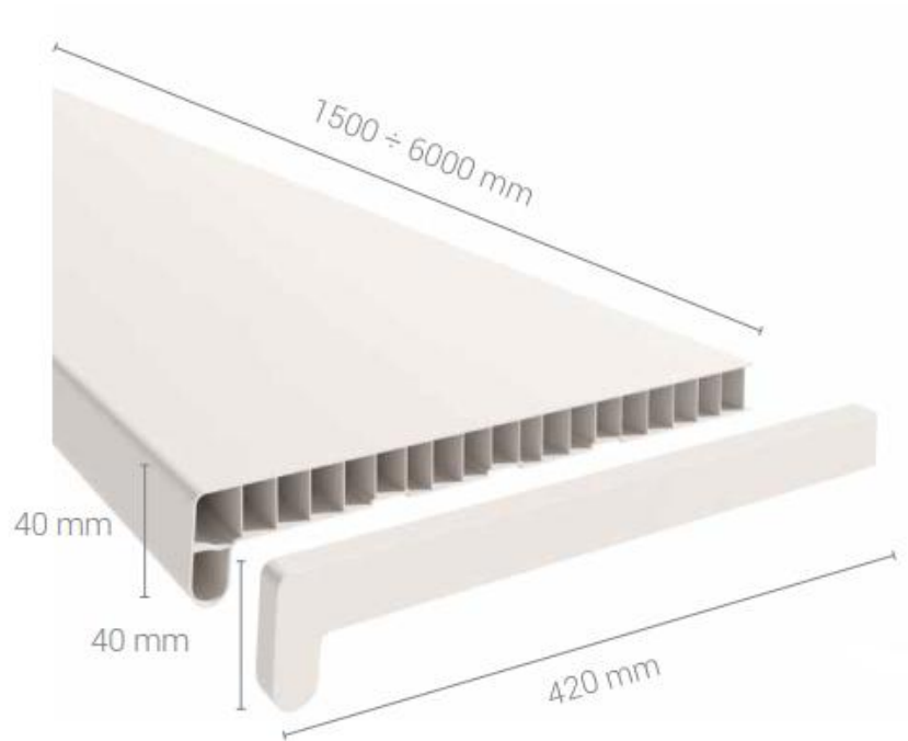
Chamber windowsill
