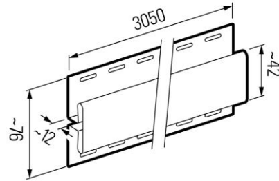
SV(P) 18 Connector
