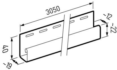
SV (P) 15 J-Trim
