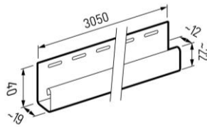
SV(P) 15 J-trim
