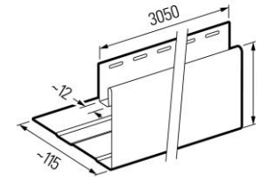
SV 17 Facade flashing small
