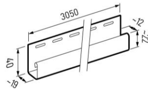
SV(P) 15 J-trim
