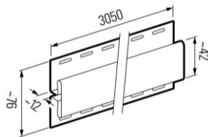
SV(P) 18 Connector
