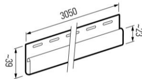
SV(P) 14 Finishing trim
