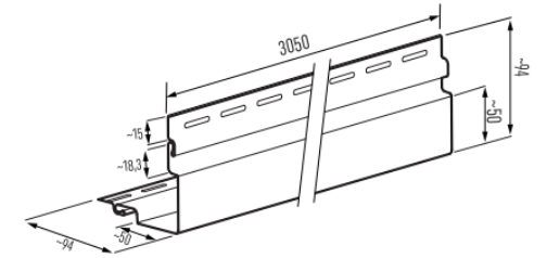
SV (P) 12V Outside corner for vertical installation
