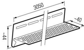
SV 11.5 Bottom ventilation trim
