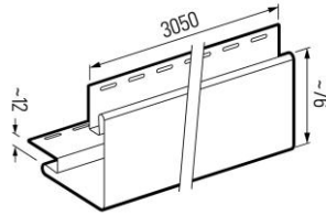
SV (P) 12 Outside corner
