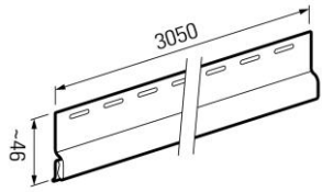
SV 11 Starting trim
